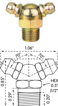
LX-3121: 1/8" PTF, 70°
