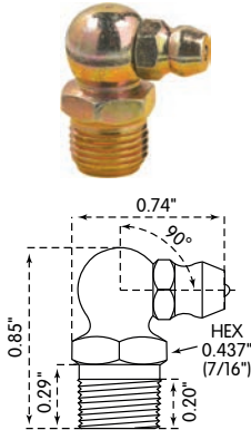
LX-3119: 1/8" PTF, 90°
