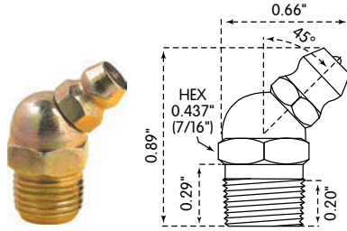
LX-3113: 1/8" PTF, 45°
