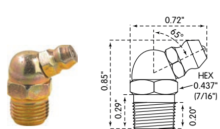
LX-3117: 1/8" PTF, 65°
