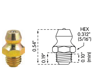
LX-3007: 1/4"-28 Taper Thread, Straight
