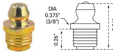
LX-3511: For 5/16" Diameter Hole, Straight
