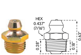
LX-3101: 1/8" PTF, Straight
