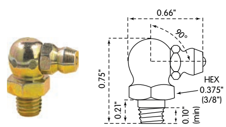
LX-3019: 1/4"-28 Taper Thread, 90°
