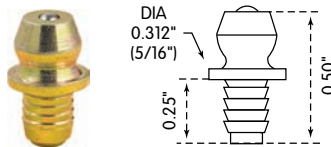
LX-3505: For 3/16" Diameter Hole, Straight
